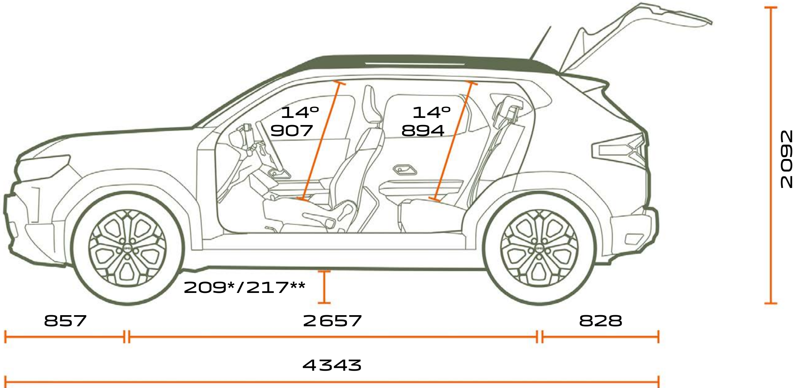
PROFILE VIEW
