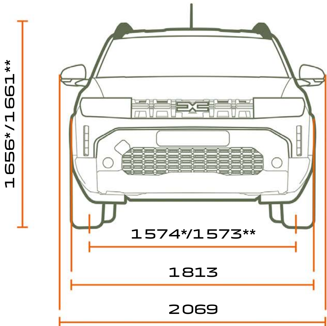
FRONT VIEW
