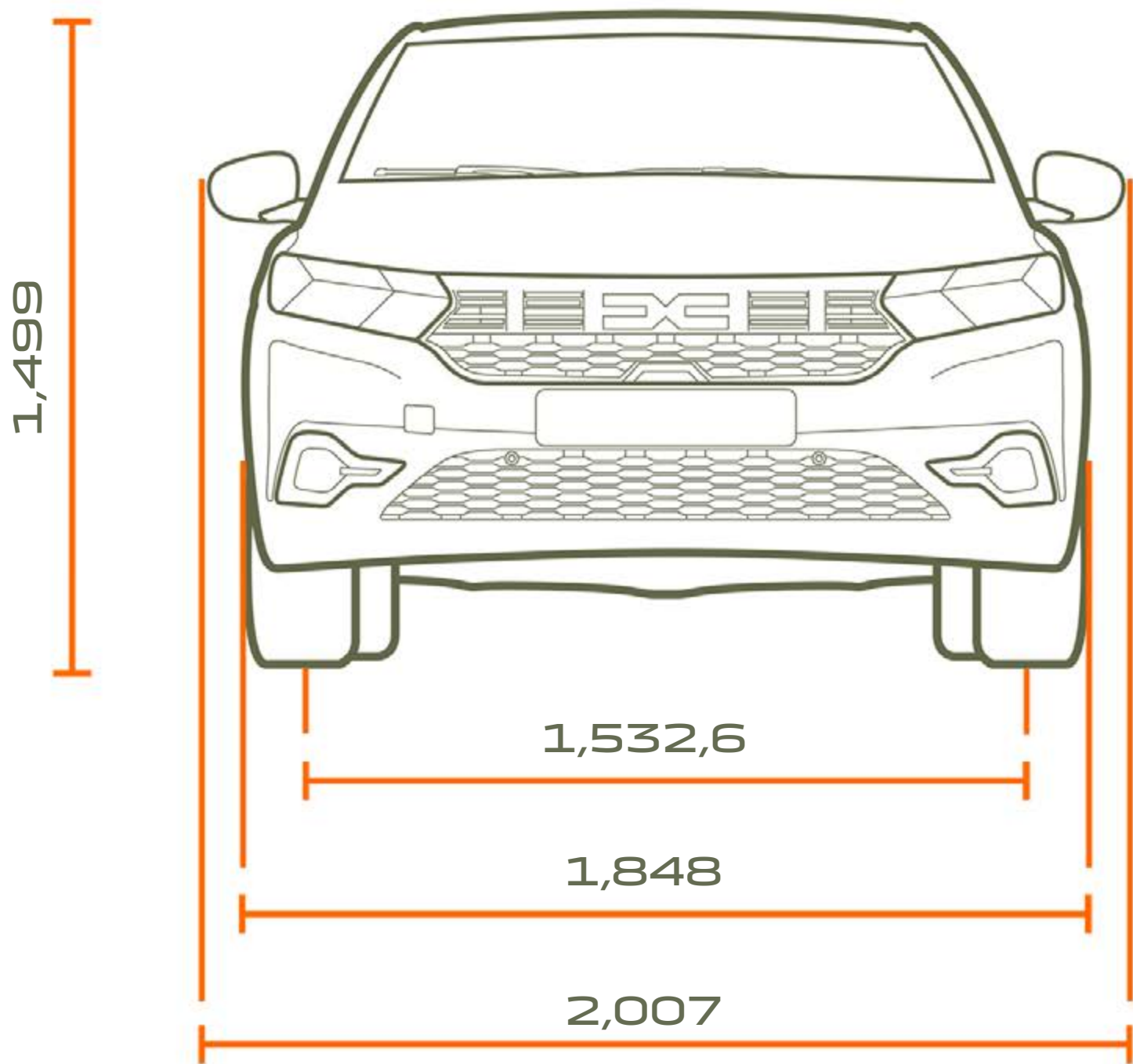
FRONT VIEW
