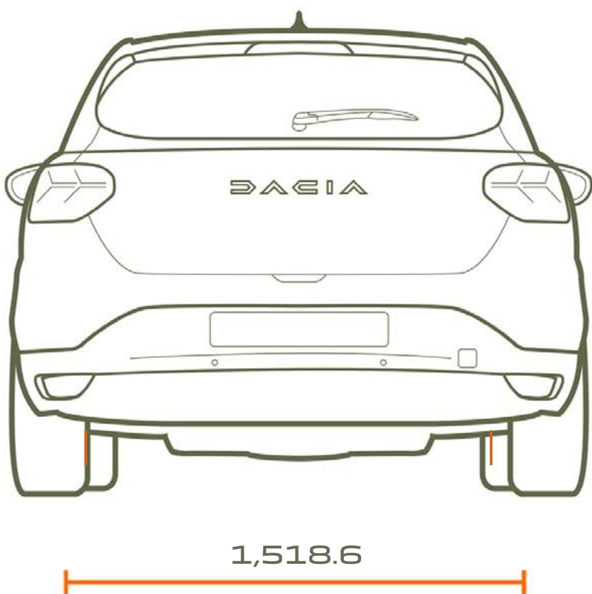
REAR VIEW
