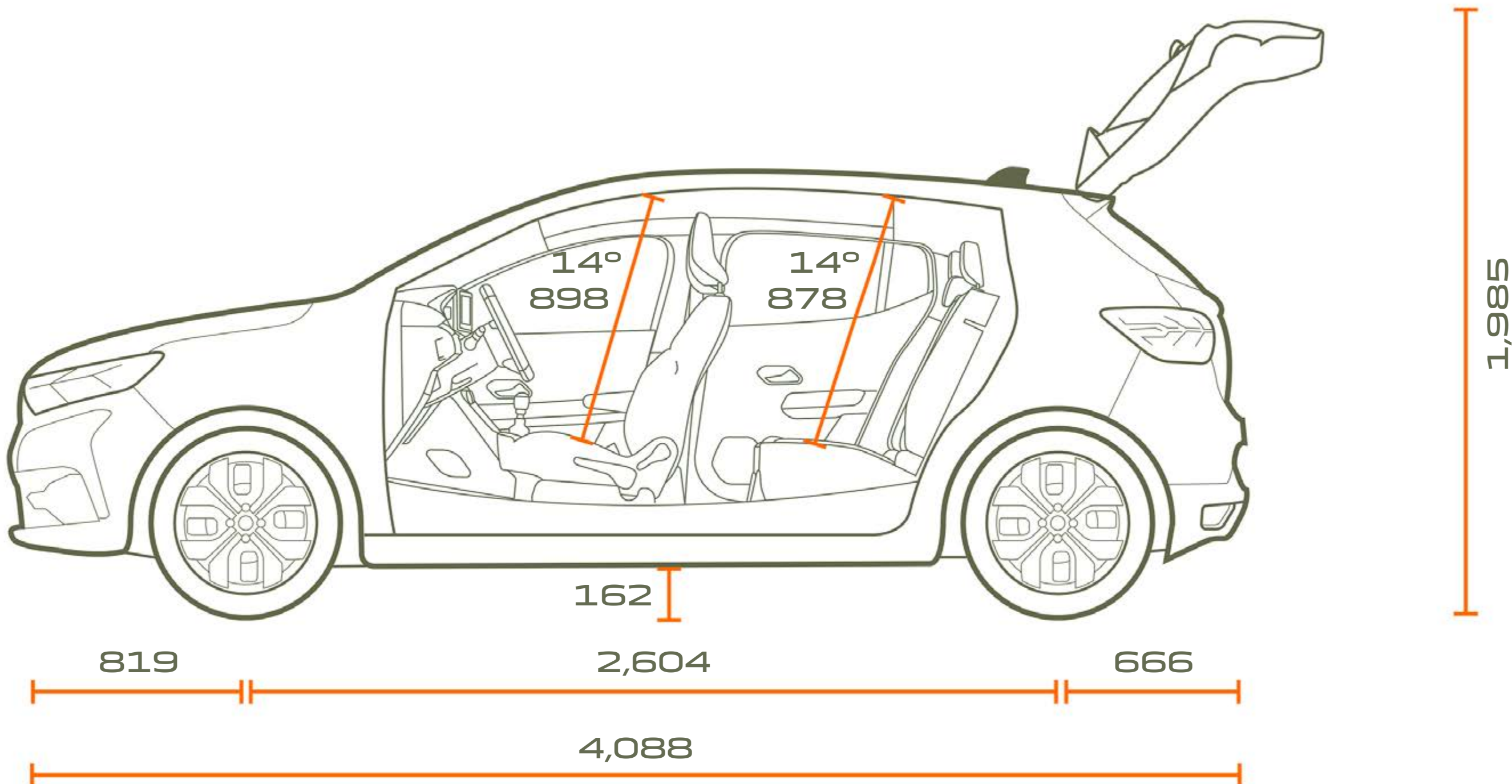
SIDE-FACE VIEW
