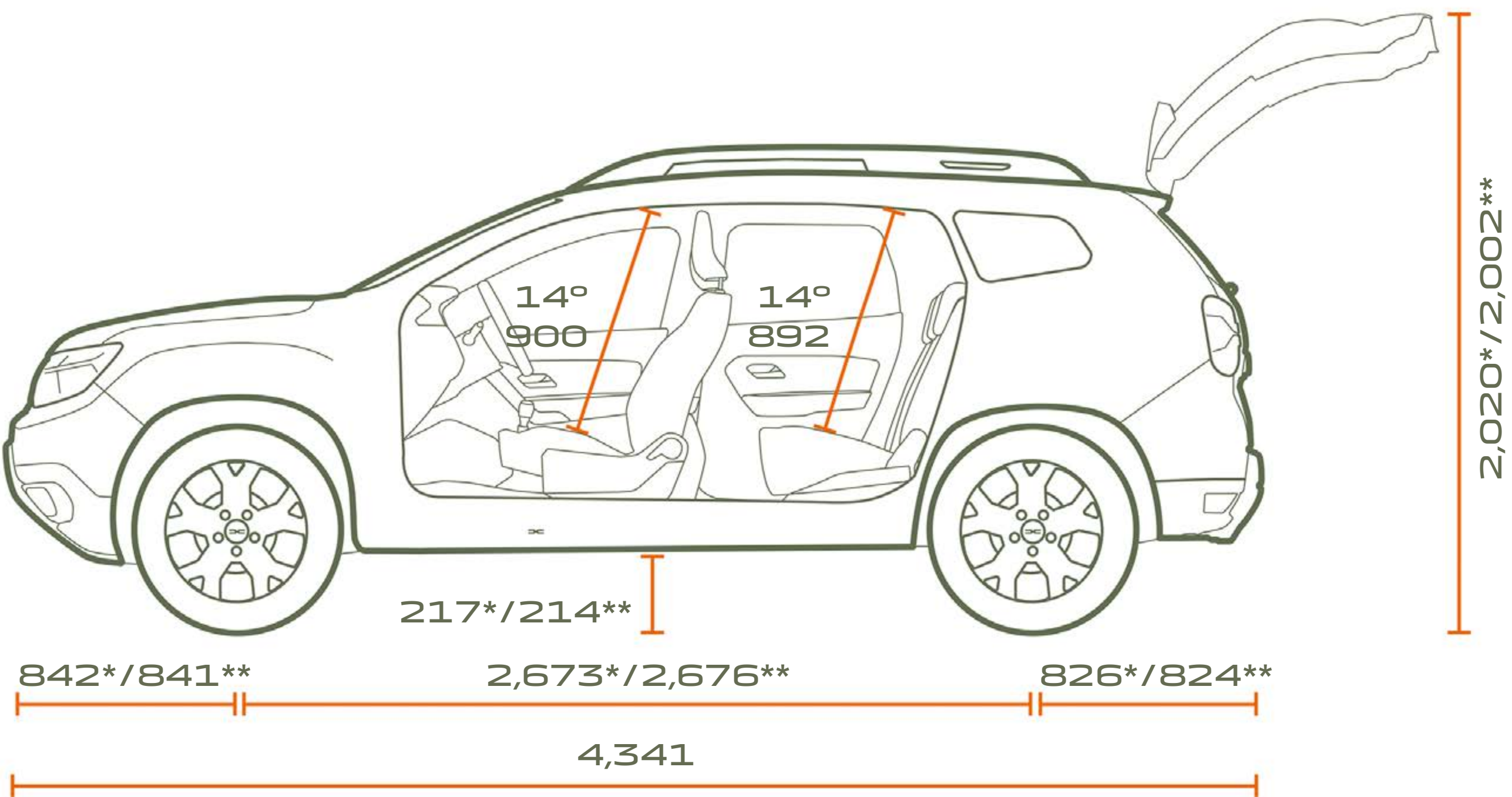
PROFILE VIEW
